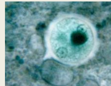
cysts of E histolytica
