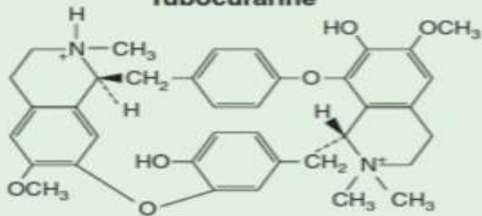
Tubocurarine
