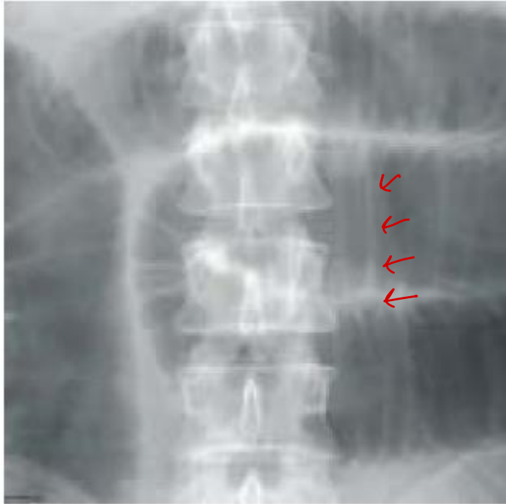
Figure 3. Valvulae conniventes
